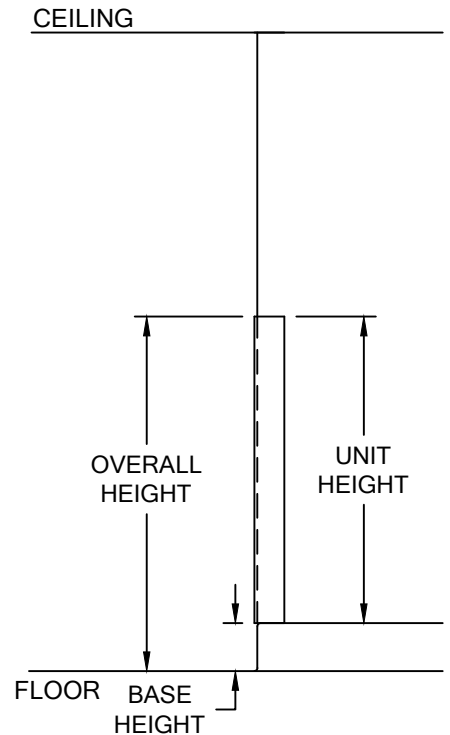
LG-250M CORNER GUARD AT PARTIAL HEIGHT ELEVATION
