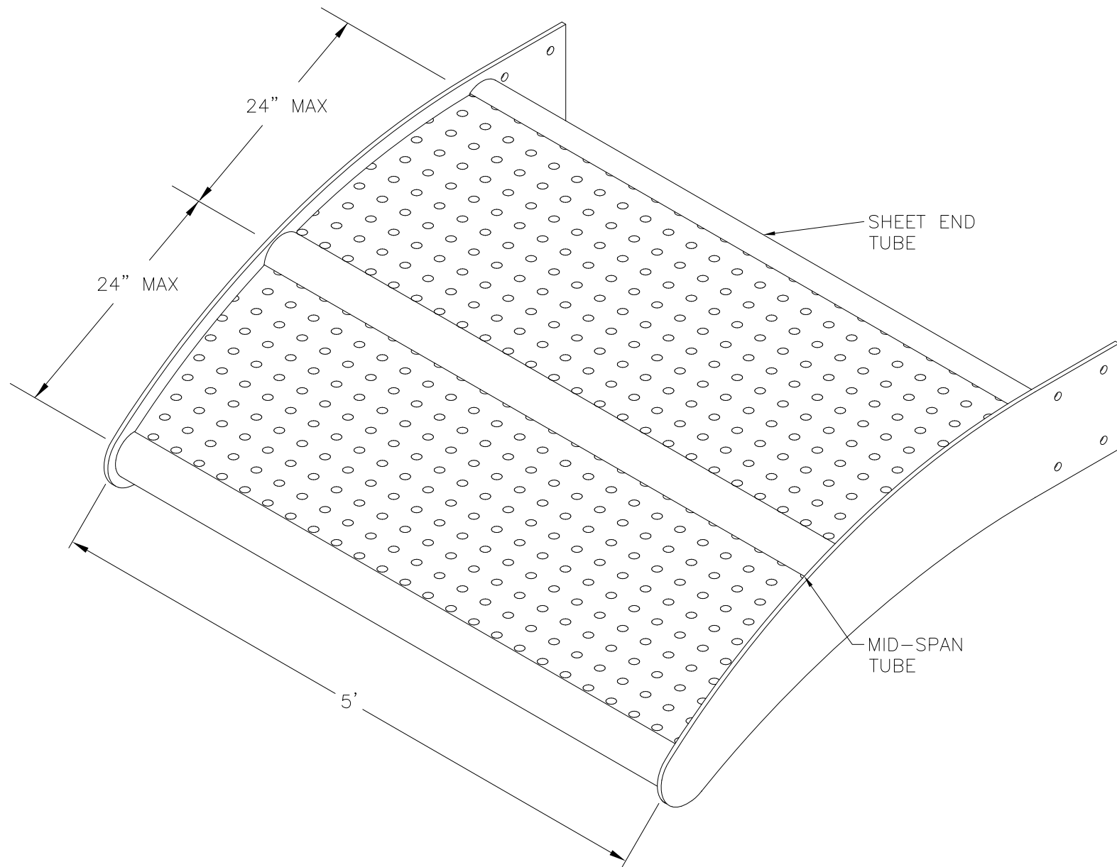
ISO VIEW WITH MID-SPAN TUBE
