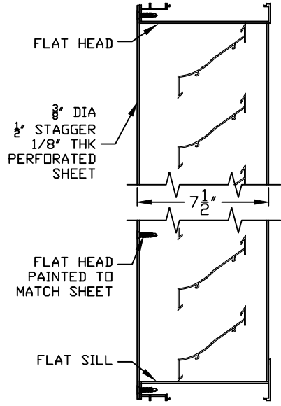
SECTION VIEW
