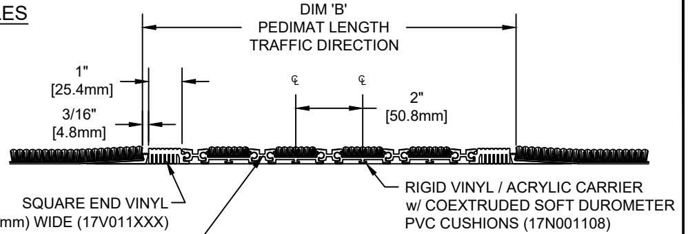
SECTION Y-Y
