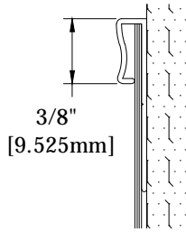
WAINSCOT TRIM (25N036XXX)
