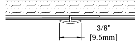
"H" JOINT MOLDING (25N033XXX)
