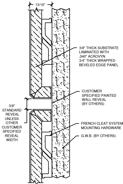
(A) PAINTED WALL REVEAL CONDITION
