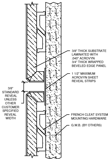
(C) ACROVYN SHEET REVEAL STRIP CONDITION
