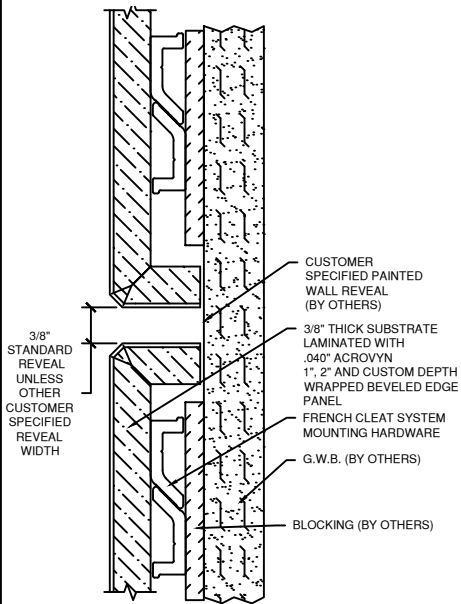
(A) PAINTED WALL REVEAL CONDITION
