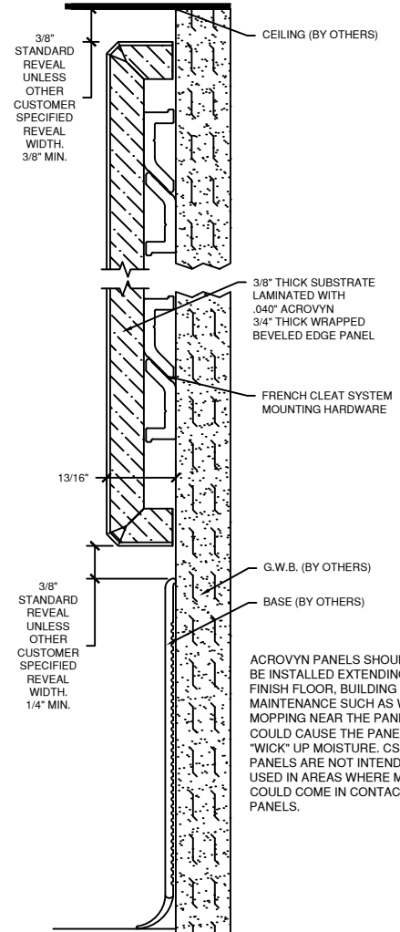
BASE AND CEILING CONDITION
