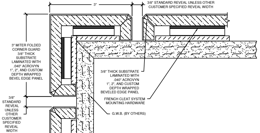
(E) MITER FOLD CORNER GUARD OPTION
