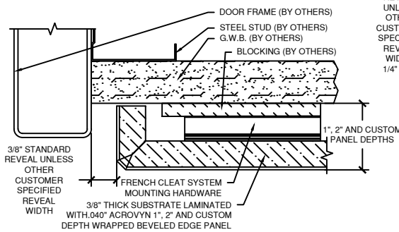
END WALL CONDITION
