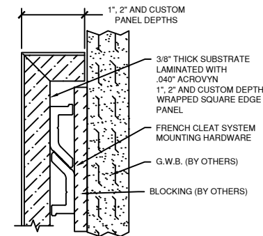
WAINSCOT CONDITION
