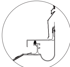
Roof to Wall
