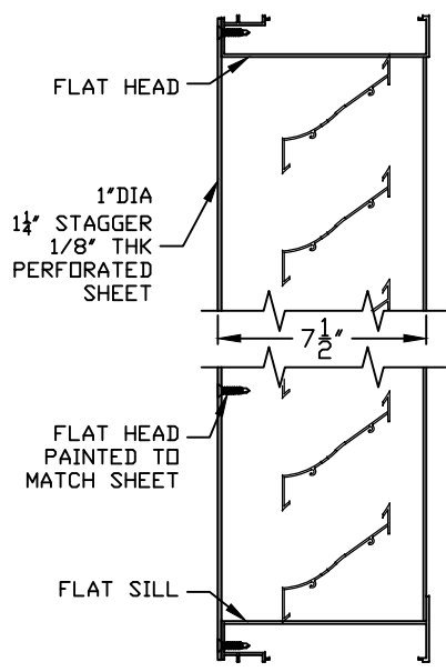
SECTION VIEW
