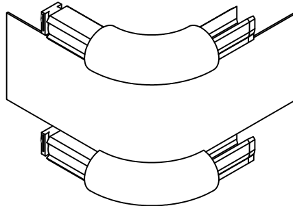
HANDRAIL OUTSIDE CORNER ASSEMBLY
