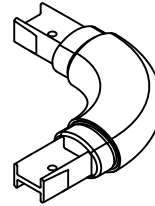
HANDRAIL INSIDE/OUTSIDE CORNER ASSEMBLY
