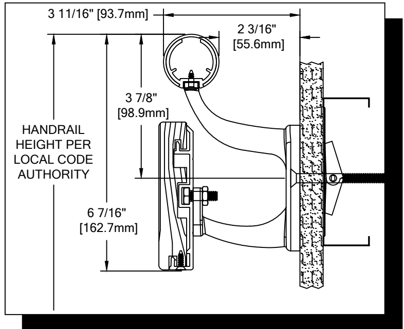
SECTIONAL VIEW *P-RAWN-INT SHOWN SEE PAGE 4 FOR P-RAWVN-INT AND P-RAWGN-INT
