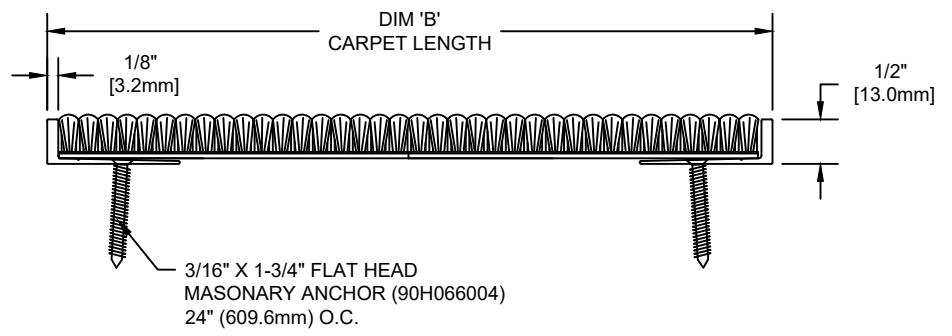
SECTION Y-Y
