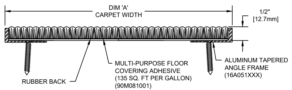
SECTION X-X
