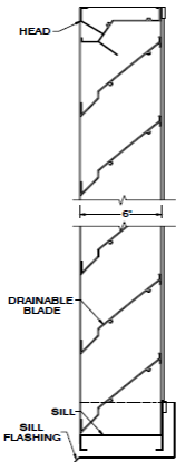
SECTION VIEW
