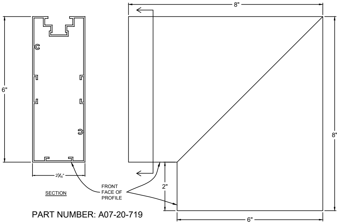
STANDARD INSIDE
