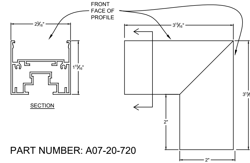
LED OUTSIDE
