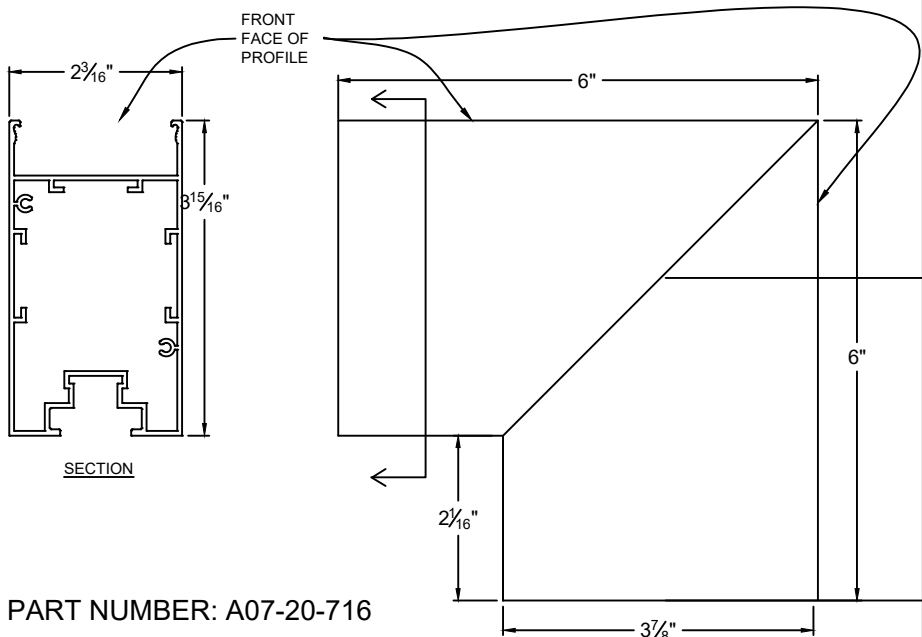
LED OUTSIDE
