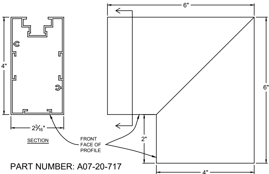
STANDARD INSIDE
