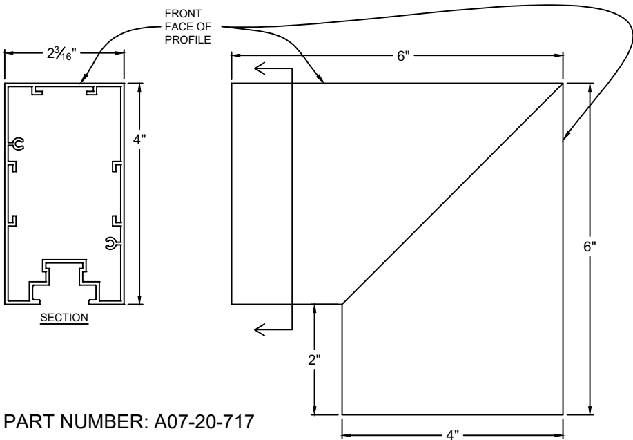
STANDARD OUTSIDE
