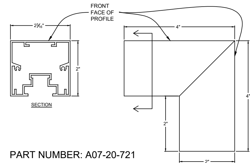
STANDARD OUTSIDE
