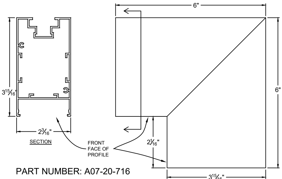
LED INSIDE
