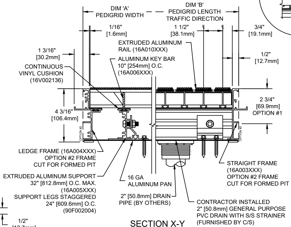
SECTION X-Y
