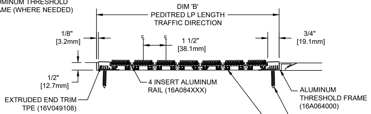
SECTION Y-Y
