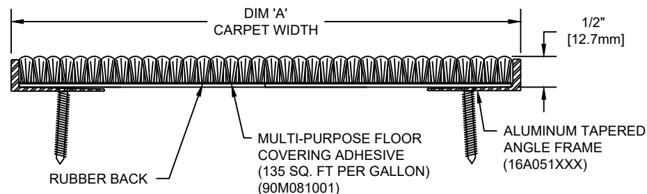
SECTION X-X
