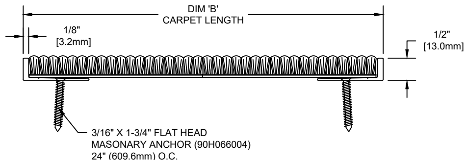
SECTION Y-Y
