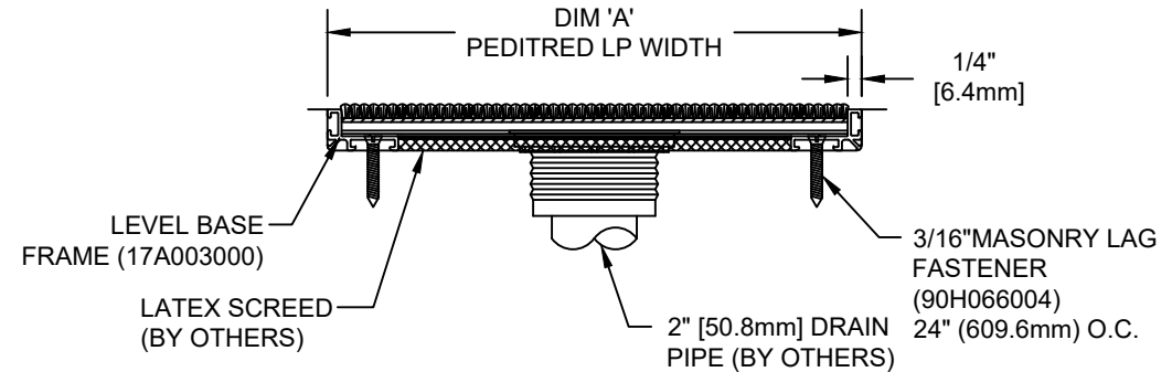
SECTION X-X
