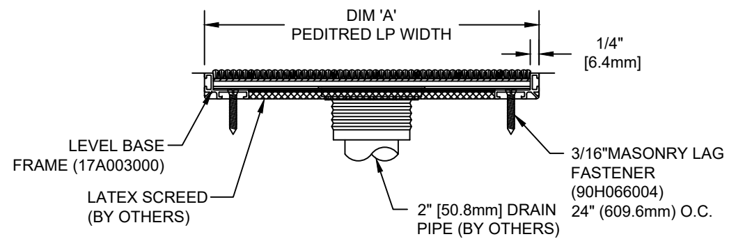
SECTION X-X
