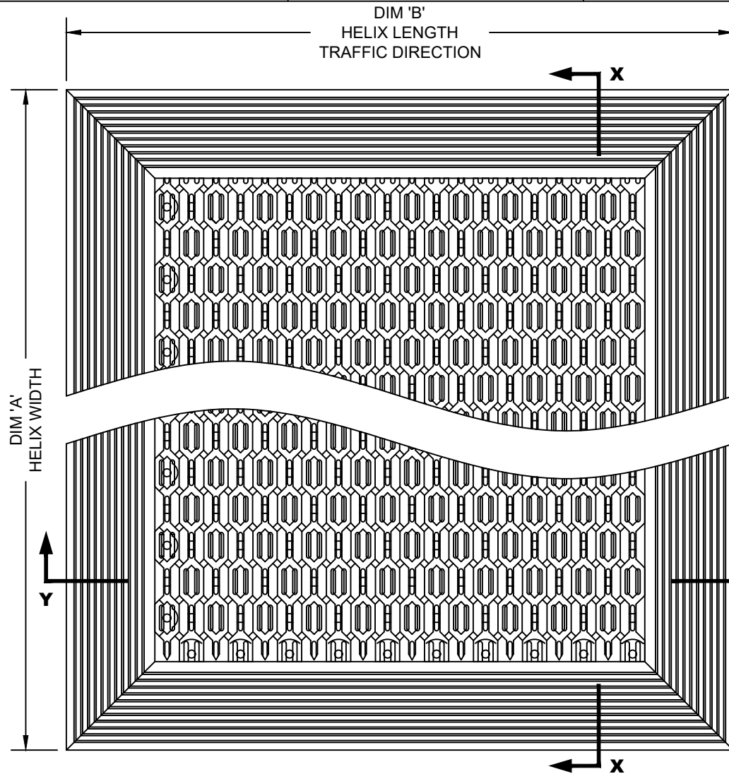
TYPICAL PLAN VIEW
