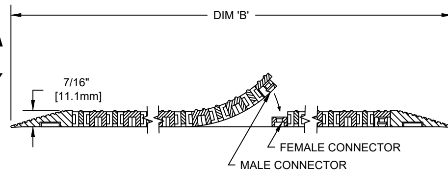
SECTION Y-Y
