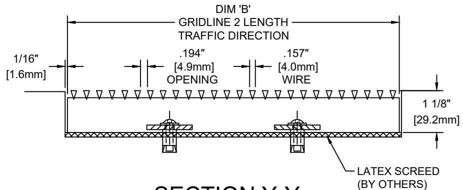
SECTION Y-Y
