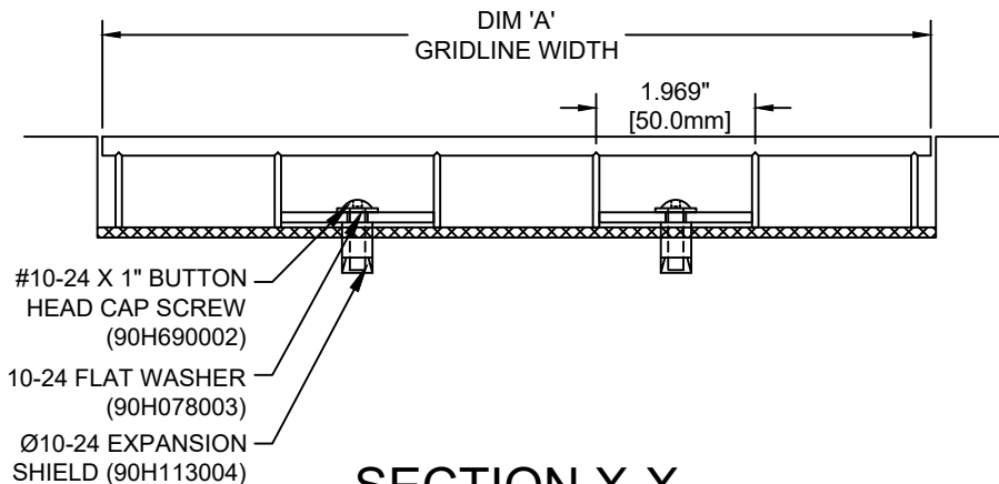
SECTION X-X
