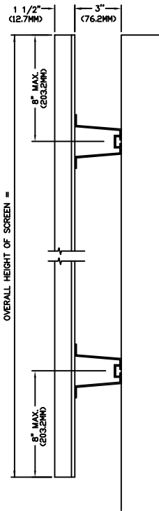
VERTICAL SECTION
