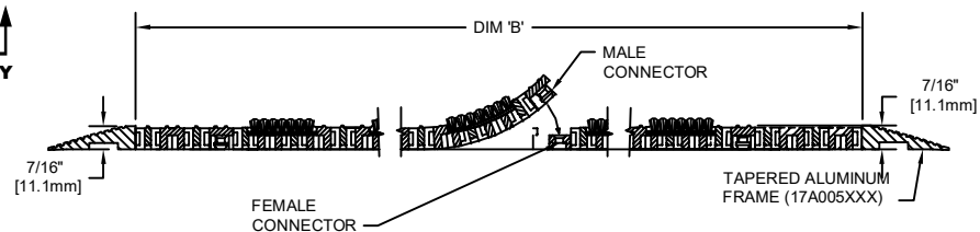
SECTION Y-Y
