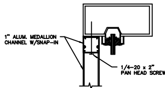
(A) SECTION
