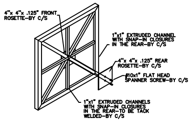
(D) TYPICAL REAR VIEW OF GRILLE SHOWING ROSETTE ATTACHMENT N.T.S.
