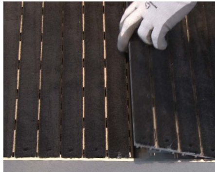
5 Join modules together by placing the aluminum foot into the black connector.
