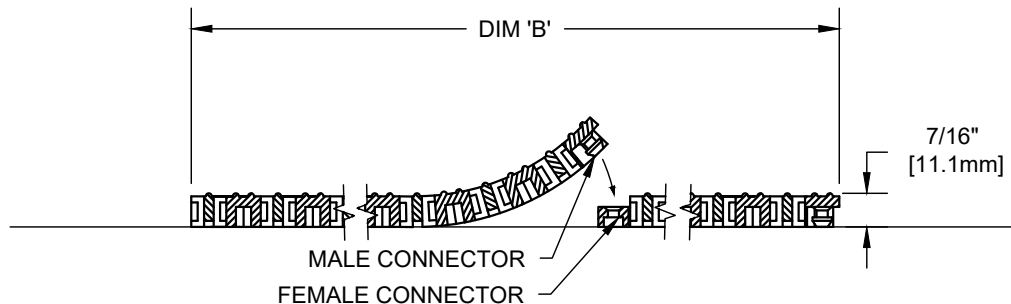
SECTION Y-Y
