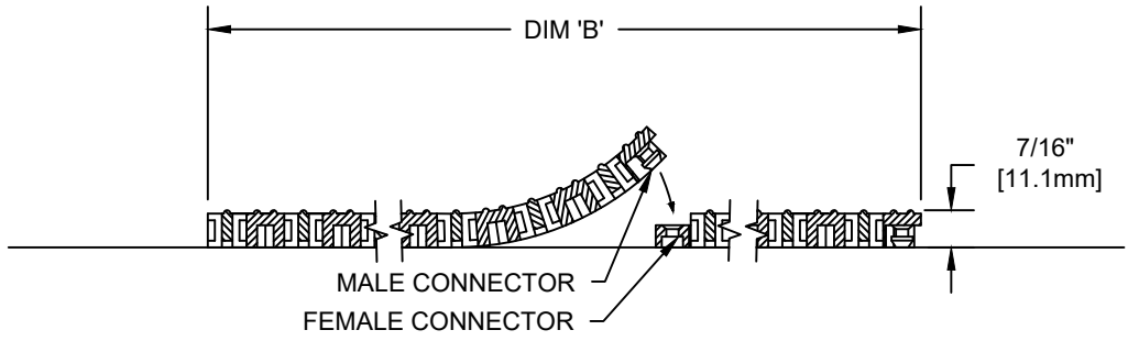
SECTION Y-Y
