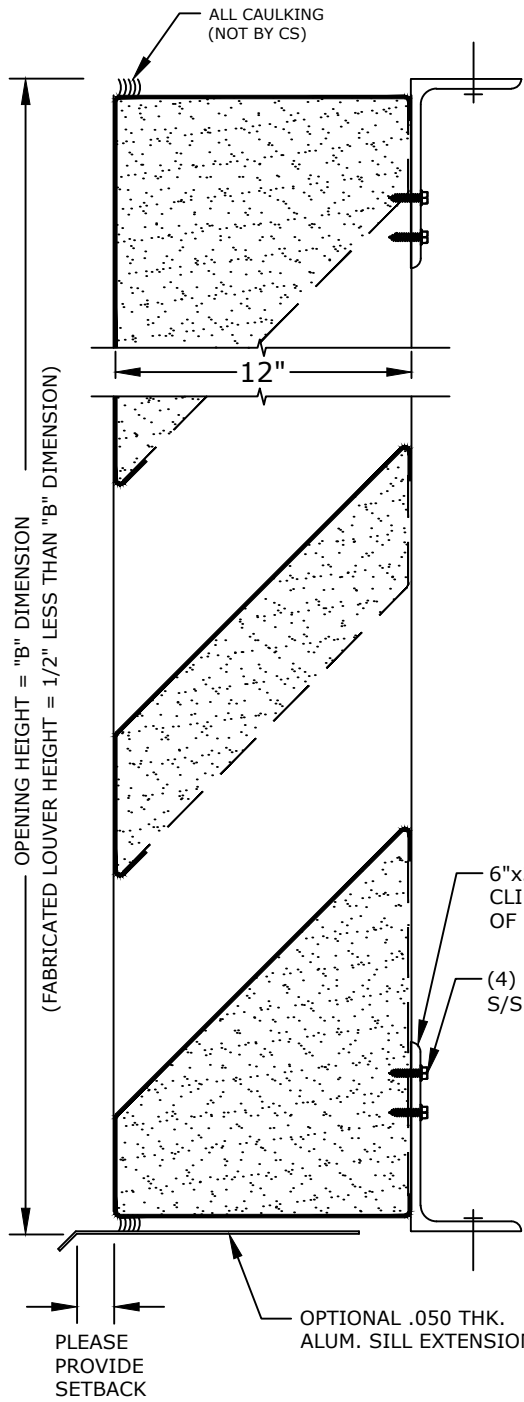
VERTICAL SECTION NTS
