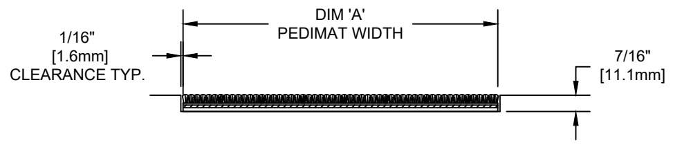
SECTION X-X
