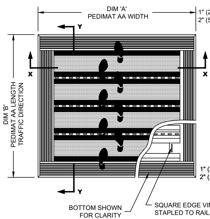
TYPICAL PLAN VIEW
