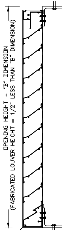
SECTION VIEW
