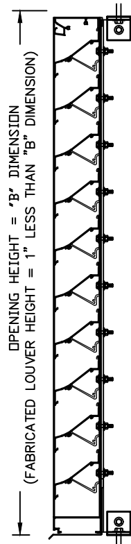
SECTION VIEW
