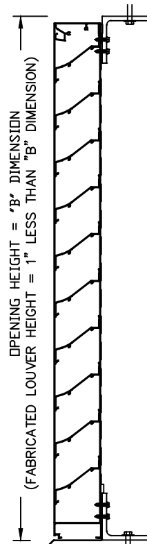
SECTION VIEW
