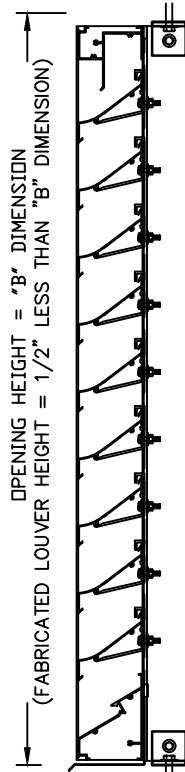
SECTION VIEW
