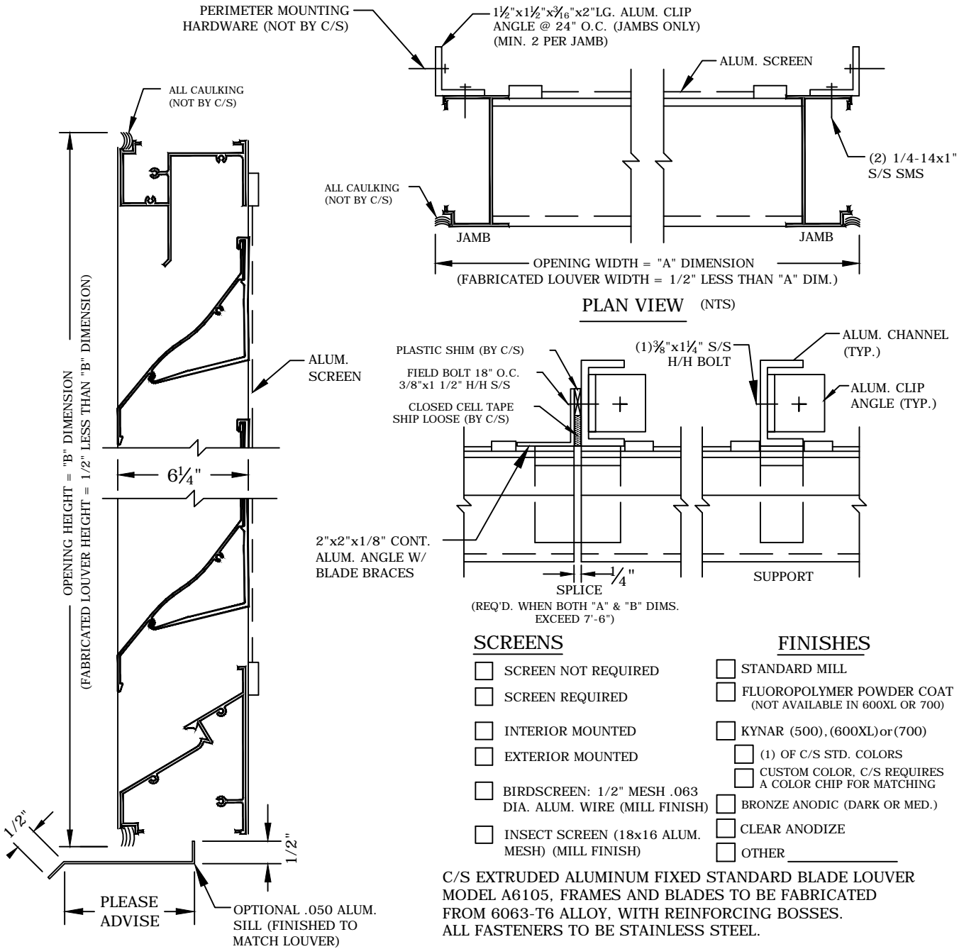
VERTICAL SECTION (NTS)
