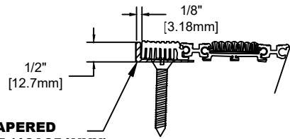
ALUMINUM TAPERED ANGLE FRAME (16A051XXX)
