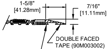
TAPERED ALUMINUM FRAME (17A005XXX)
