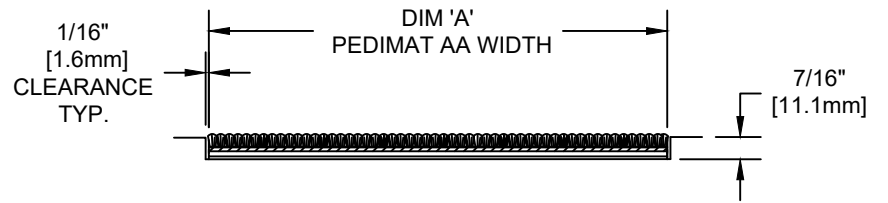
SECTION X-X
