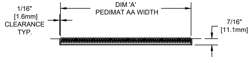
SECTION X-X
