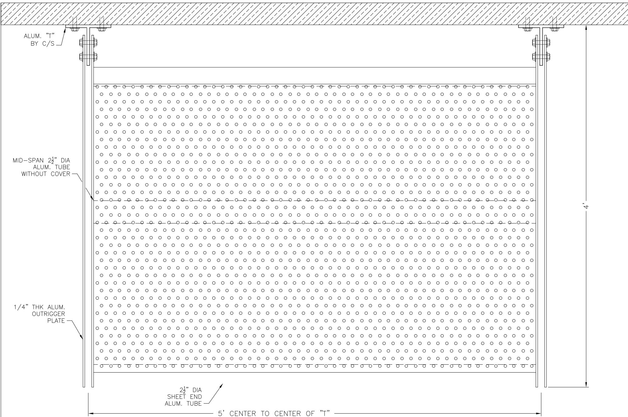
PLAN VIEW WITH MID-SPAN TUBE
