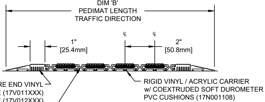
SECTION Y-Y
