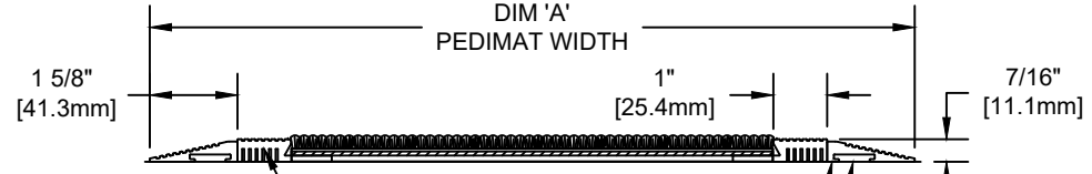
SECTION X-X
