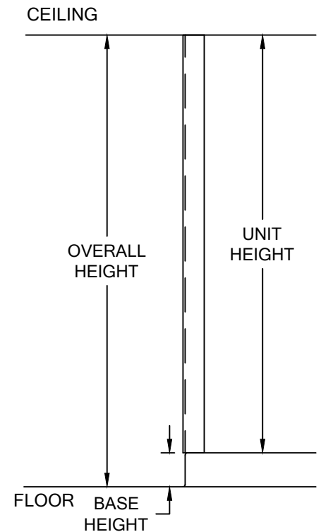
LG-200M CORNER GUARD AT FULL HEIGHT ELEVATION
