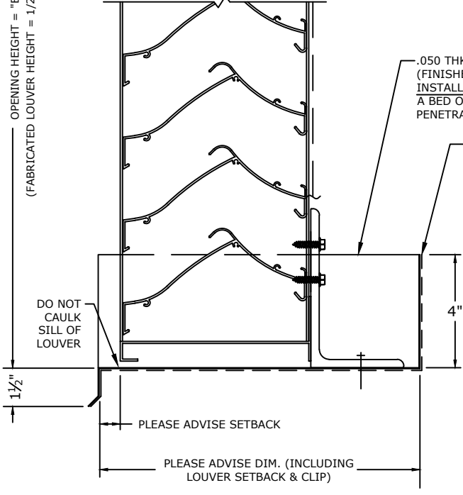
VERTICAL SECTION (NTS)
