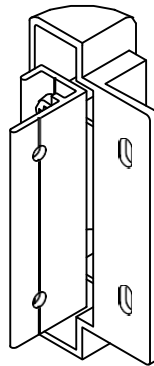
CRASH RAIL OUTSIDE CORNER ASSEMBLY (SCR40OSxxx)
