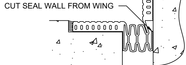
END VIEW
