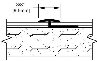
VERTICAL JOINT TRIM (25N033xxx)
