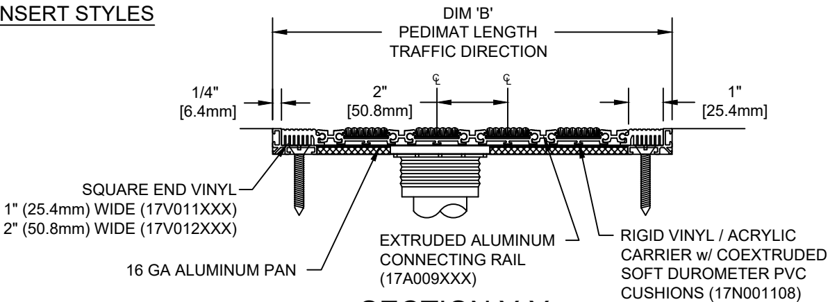
SECTION Y-Y
