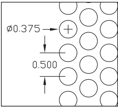
3/8" Hole (9.5mm)
