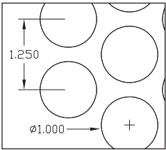
1" Hole (25.4mm)
