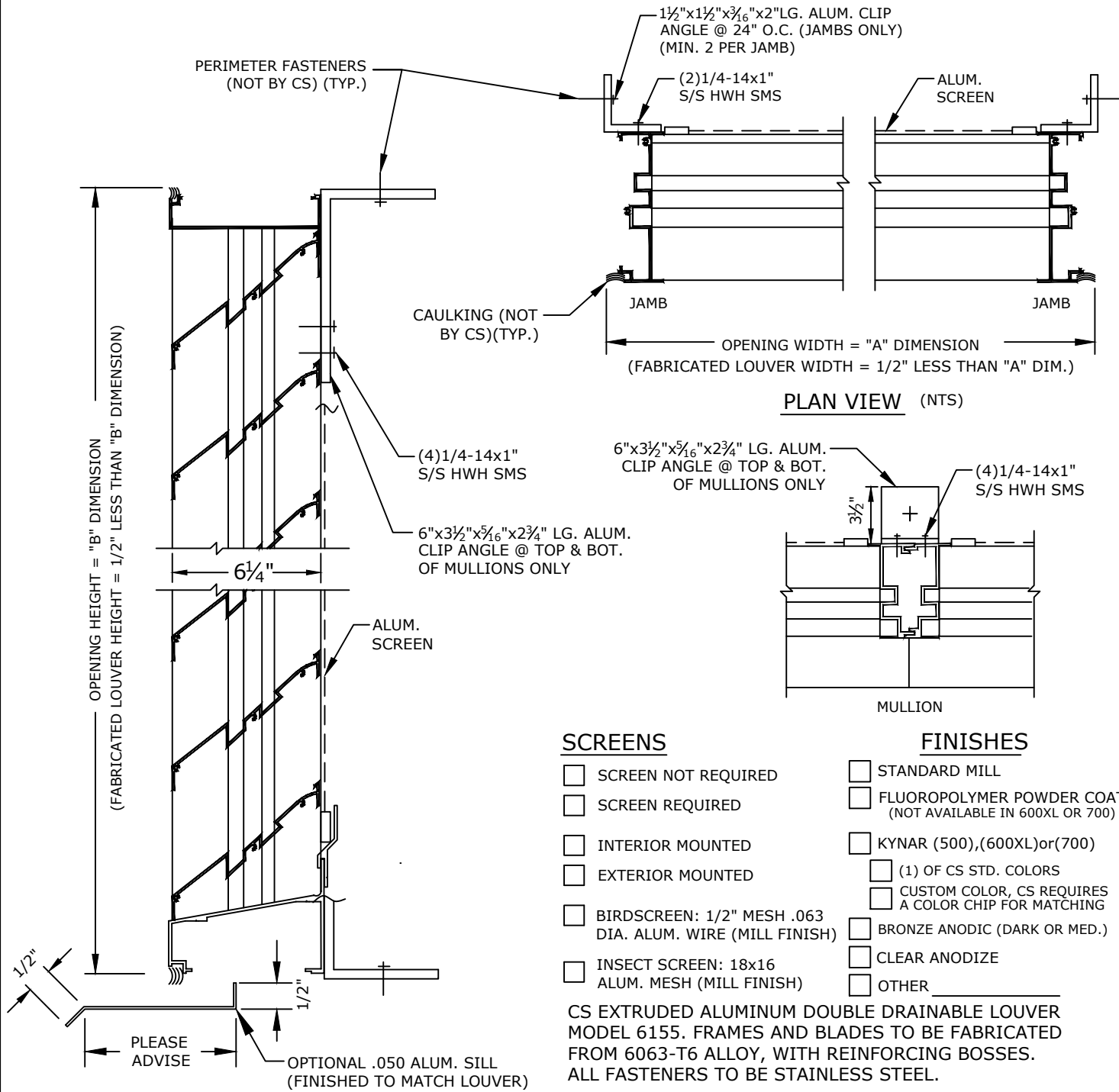
VERTICAL SECTION (NTS)
