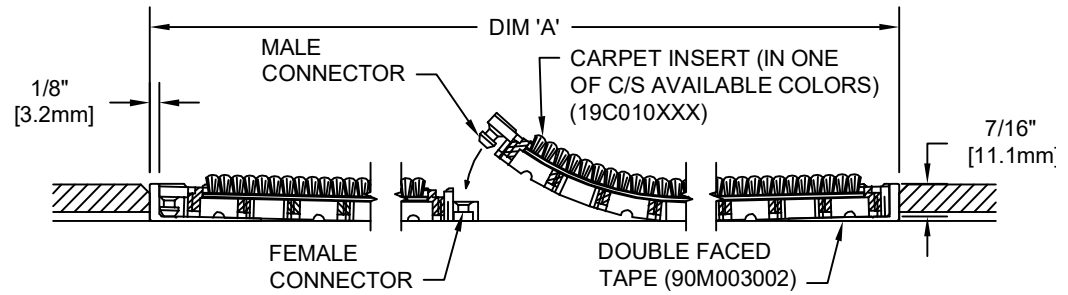
SECTION X-X
