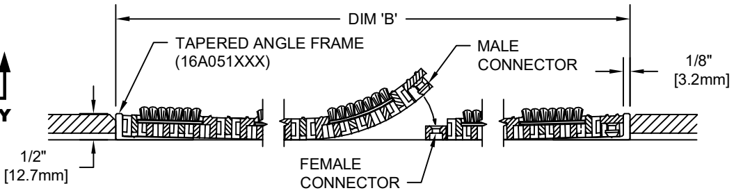
SECTION Y-Y
