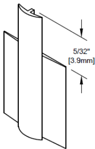
Rabbet Detail Metal vertical trim shown. Metal inside/outside corner trims also to be rabbeted.
