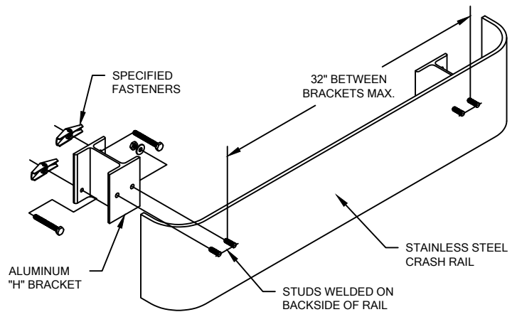
TYPICAL ASSEMBLY
