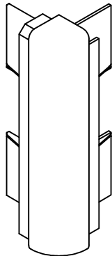
CRASH RAIL OUTSIDE CORNER ASSEMBLY
