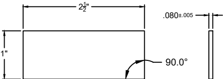
SPLICE PLATE 08-01-380
