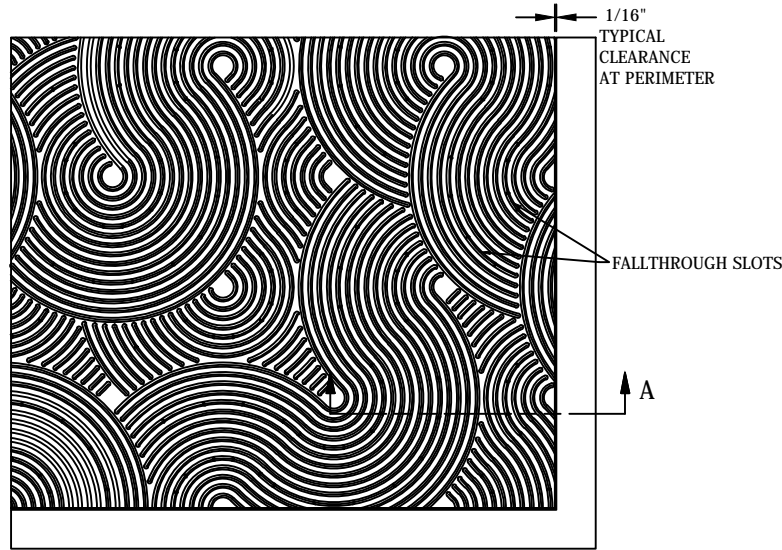
PLAN VIEW SCALE 1:5
