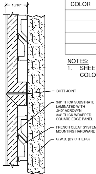
(B) BUTTED PANEL CONDITION
