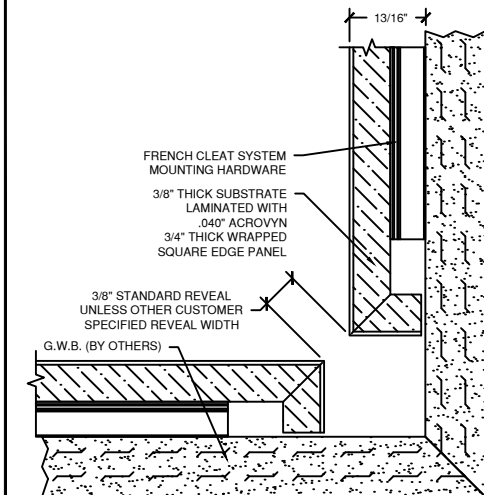
(F) INSIDE CORNER WITH REVEAL OPTION
