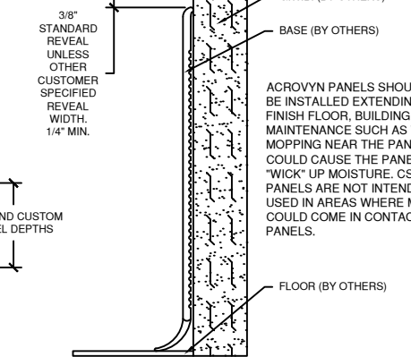
BASE AND CEILING CONDITION
