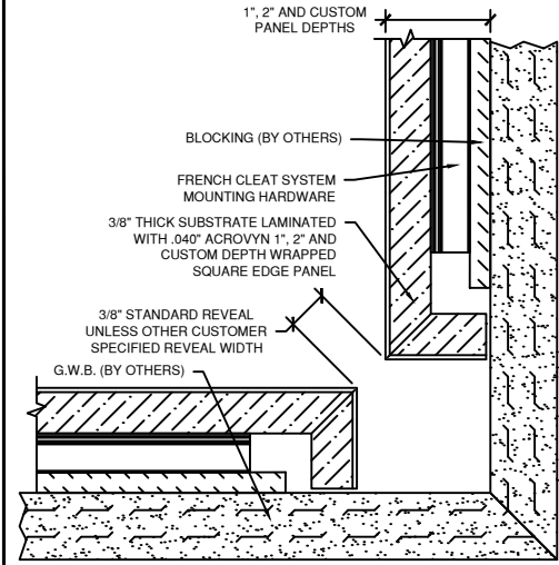
(F) INSIDE CORNER WITH REVEAL OPTION
