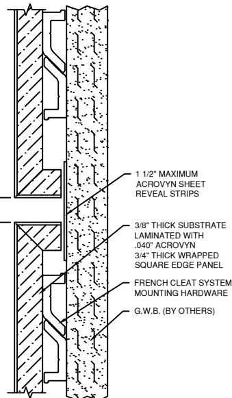
(C) ACROVYN SHEET REVEAL STRIP CONDITION
