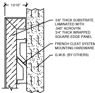
WAINSCOT CONDITION
