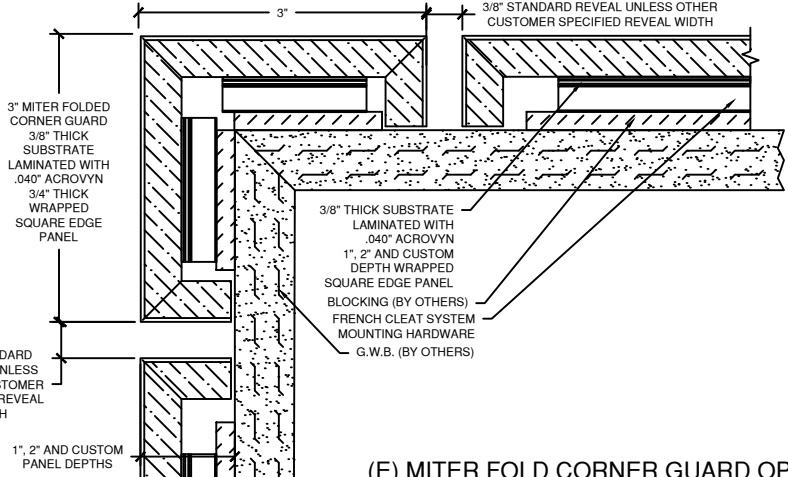
(E) MITER FOLD CORNER GUARD OPTION
