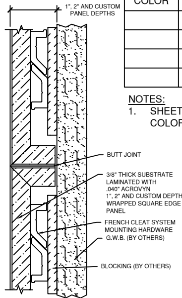
(B) BUTTED PANEL CONDITION
