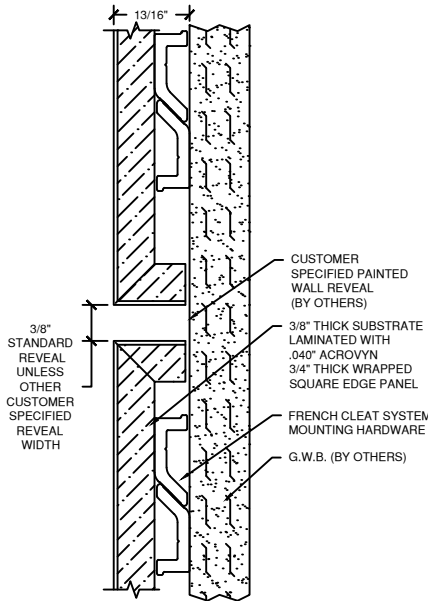
(A) PAINTED WALL REVEAL CONDITION
