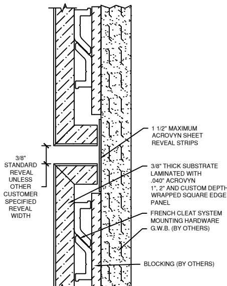
(C) ACROVYN SHEET REVEAL STRIP CONDITION
